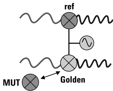
Figure 8. A golden mixer is one method used to normalize a test system and perform relative measurements.
